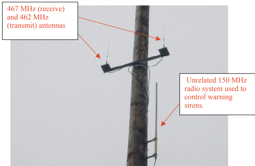
Top: DCU at Sloat Boulevard and 47th Avenue.
