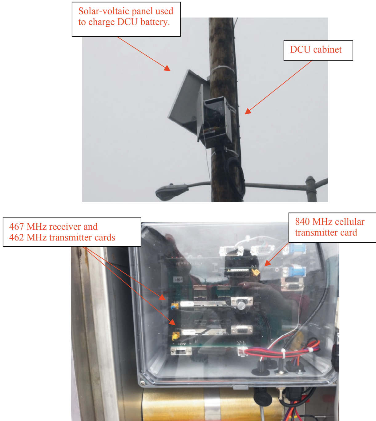
Top: Pole-mounted DCU and solar-voltaic panel. Bottom: DCU modules.
