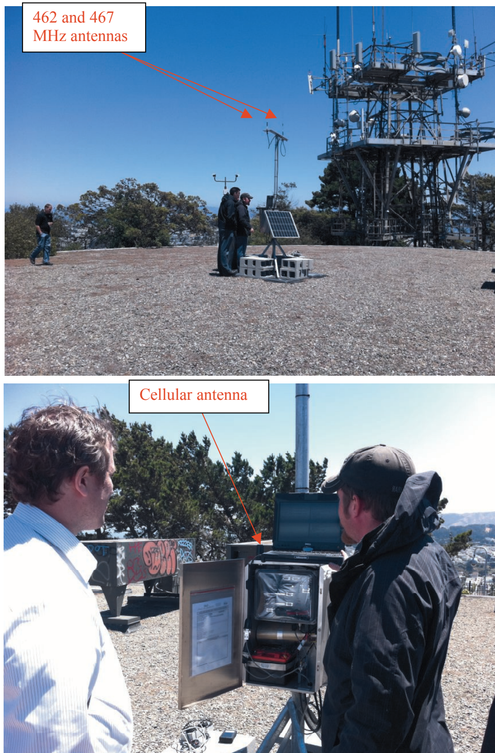
Top: DCU on roof of the Bernal Heights radio site building at 99 Moultrie Street. Bottom: DCU cabinet, with 838 MHz cellular and 462 MHz transmitters.
