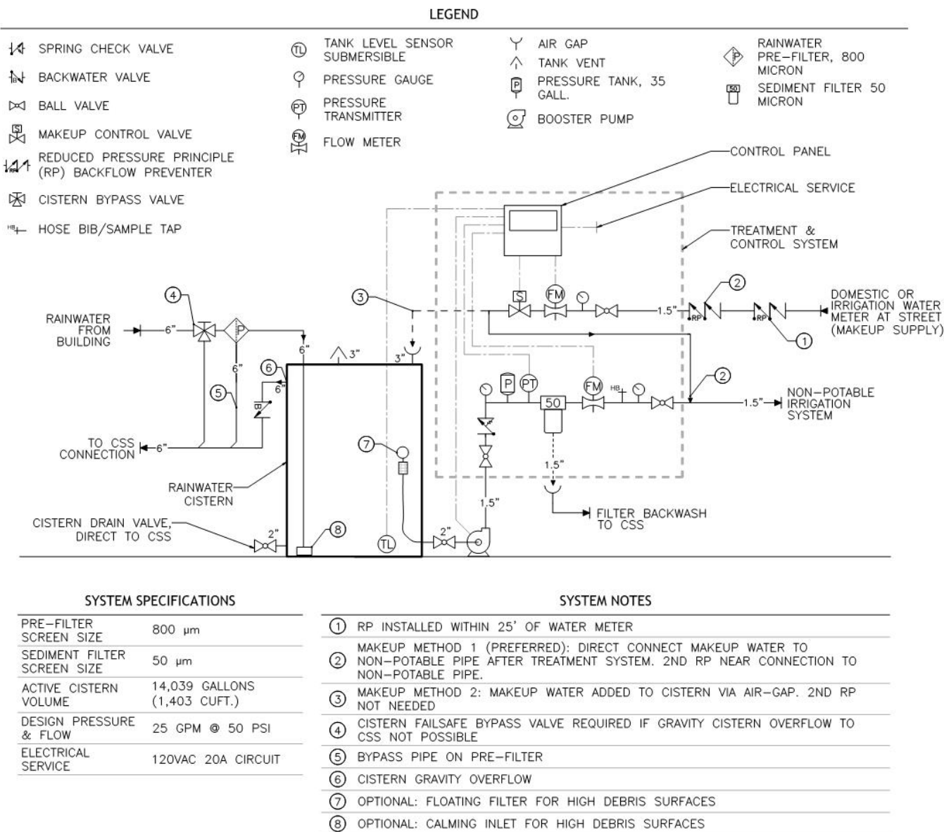
Figure 4a. RWH System Schematic Diagram Example
