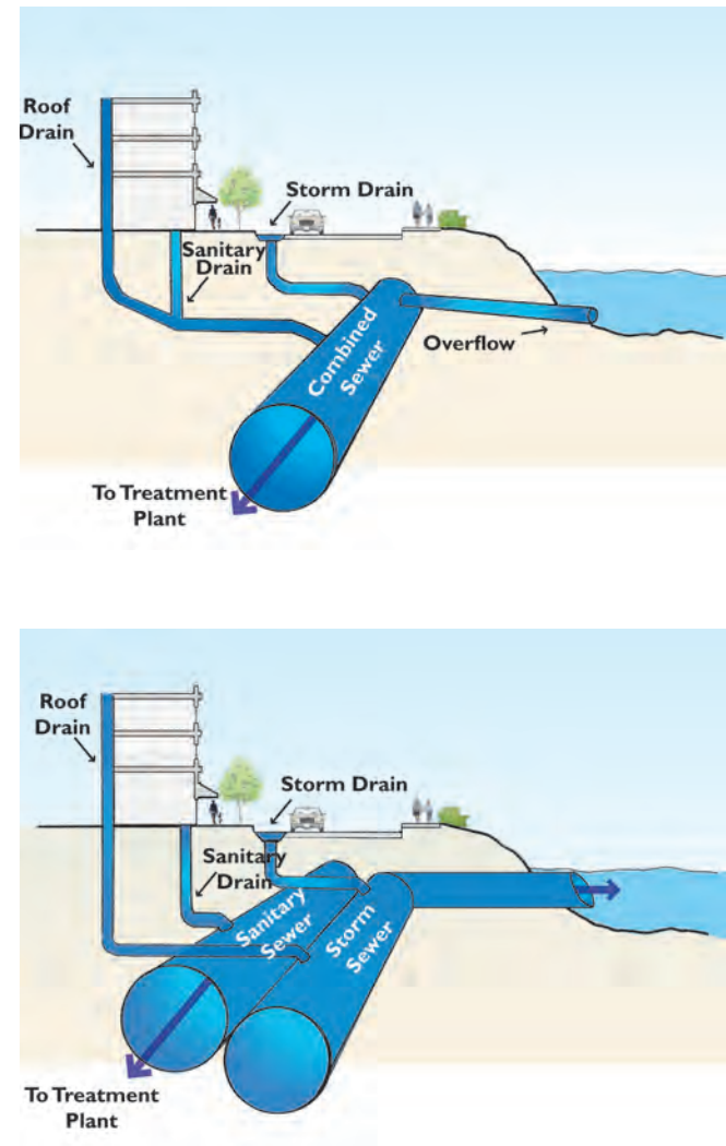
Figure 5. Combined sewer systems (top) serve 90 percent of San Francisco. Separate sewer systems (bottom) serve 10 percent. Image: modified from King County Wastewater Management Division
